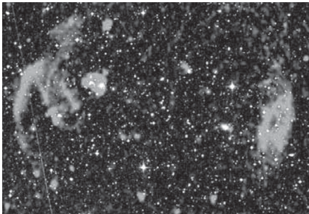
Figura 1.2 - Big-bang (Fonte: http://space.newscientist.com ).
