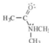
N,N-Dimetilacetamida
