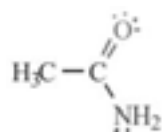
Acetamida
